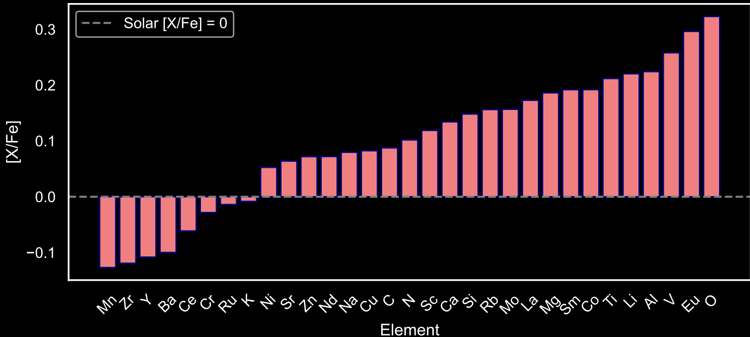
Abundance Pattern for GALAH Red Giants: Star Field [11] (N=58)
