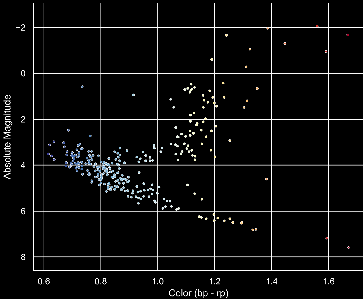
GALAH Hertzprung-Russel Diagram Field [11] Ra [328.28] Dec [-53.74]
