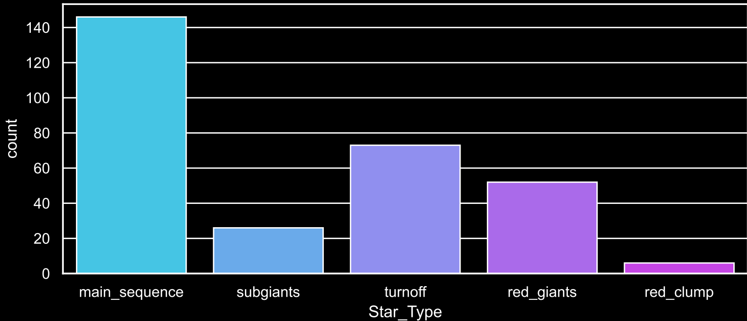
Field [11] Count plot of Star Type
