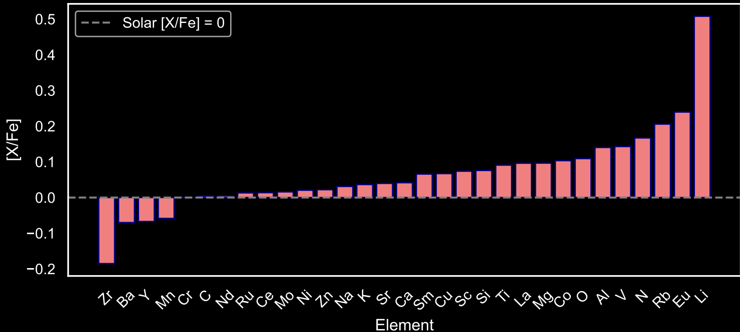
Abundance Pattern for GALAH Star Field [11] (N=303)
