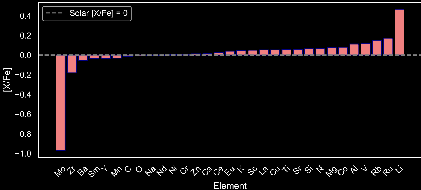
Abundance Pattern for GALAH Main Sequence Stars: Star Field [11] (N=146)
