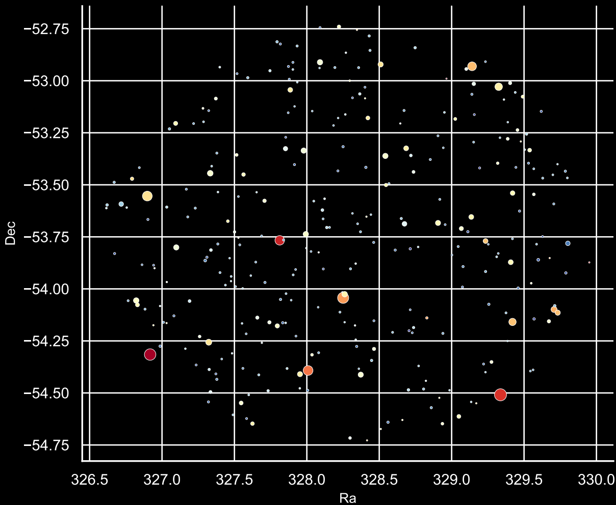
Field [11] Ra [328.28] Dec [-53.74] Stars: 303
